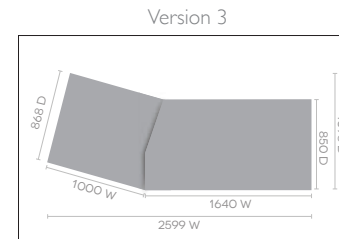
Accent Service Desk (Seated & Standing Workspace) ACCENTV3L (VERSION 3) 740-920 H X 2599 W X 1098 D
